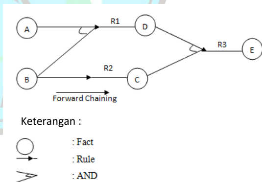
Gambar 2. Rule dasar Forward Chaining
