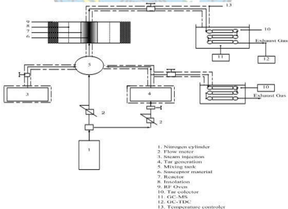
Gambar 2. Sketsa diagram peralatan percobaan
