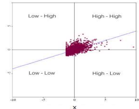
Gambar 1 Moran scatterplot
